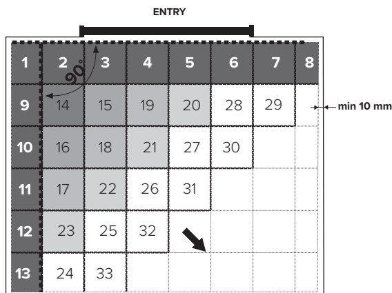
Fig. 2 Installing Fortelock INVISIBLE, INVISIBLE XL, BUSINESS
