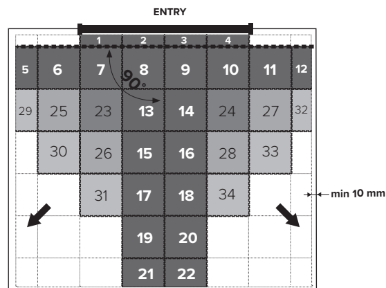
Fig. 1 Installing Fortelock INDUSTRY, INDUSTRY ULTRA, XL
