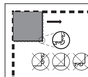
Fig. 3 Direction of installing INVISIBLE, INVISIBLE XL, BUSINESS
