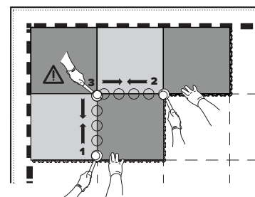
Fig. 4 Method of installing INVISIBLE, INVISIBLE XL, BUSINESS
